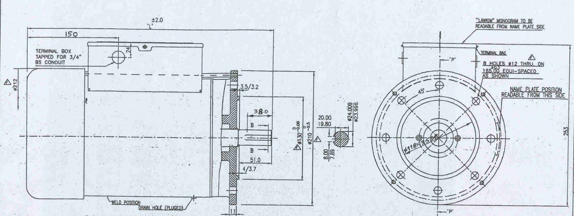
PARTIAL - SECTION - 'P-P'
